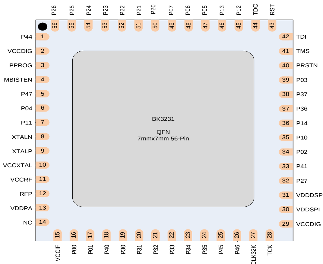
Figure 2BK3231QFN56Pin Assignment
