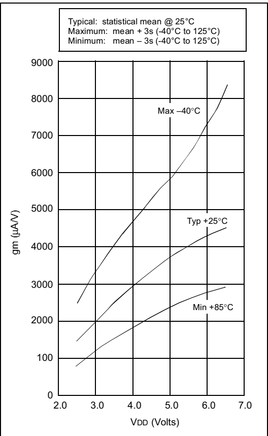
FIGURE 14-16: TRANSCONDUCTANCE (gm) OF HS OSCILLATOR vs. VDD
