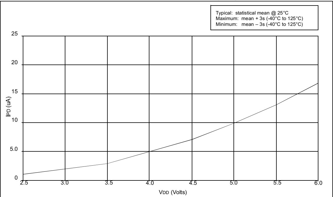
FIGURE 18-6: TYPICAL I_{PD} vs. V_{DD} , WATCHDOG ENABLED (25°C)
