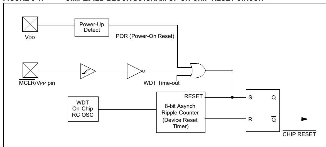
FIGURE 5-1: SIMPLIFIED BLOCK DIAGRAM OF ON-CHIP RESET CIRCUIT
