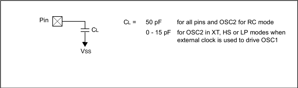
FIGURE 12-1: LOAD CONDITIONS FOR DEVICE TIMING SPECIFICATIONS - PIC16C54/55/56/57
