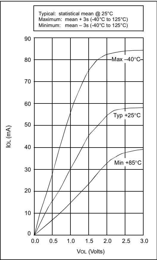
FIGURE 20-9: I_{OL} vs. V_{OL} , V_{DD} = 5\text{ V}
