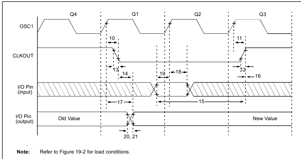
FIGURE 19-4: CLKOUT AND I/O TIMING - PIC16C5X-40
