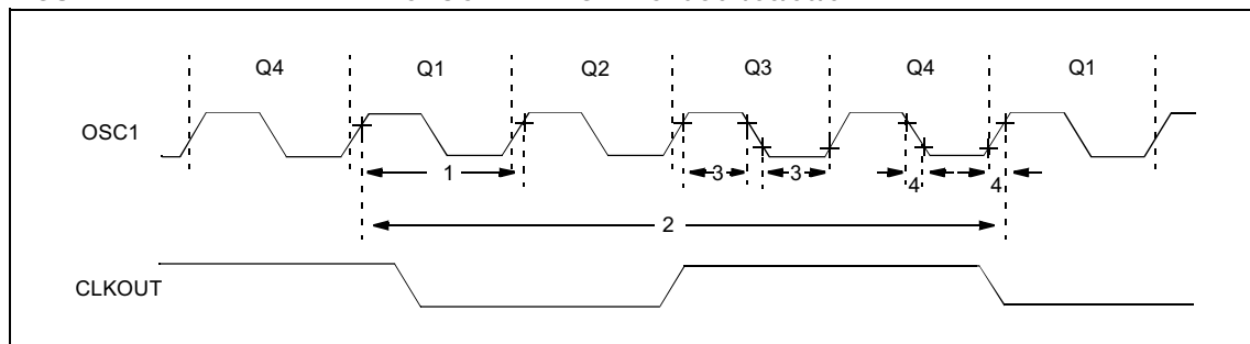
FIGURE 12-2: EXTERNAL CLOCK TIMING - PIC16C54/55/56/57
