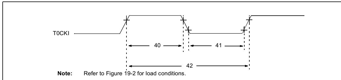
FIGURE 19-6: TIMER0 CLOCK TIMINGS - PIC16C5X-40
