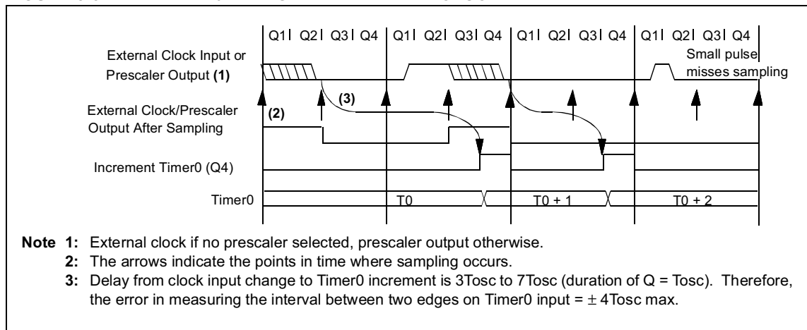
FIGURE 8-5: TIMER0 TIMING WITH EXTERNAL CLOCK
