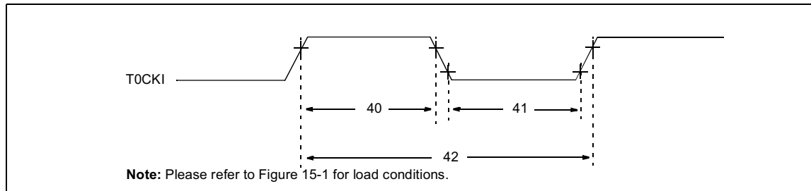
FIGURE 15-5: TIMER0 CLOCK TIMINGS - PIC16C54A
