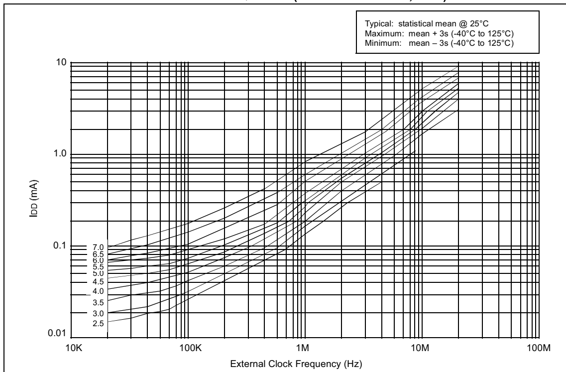
FIGURE 14-12: TYPICAL I_{DD} VS. FREQUENCY (EXTERNAL CLOCK, 25°C)
