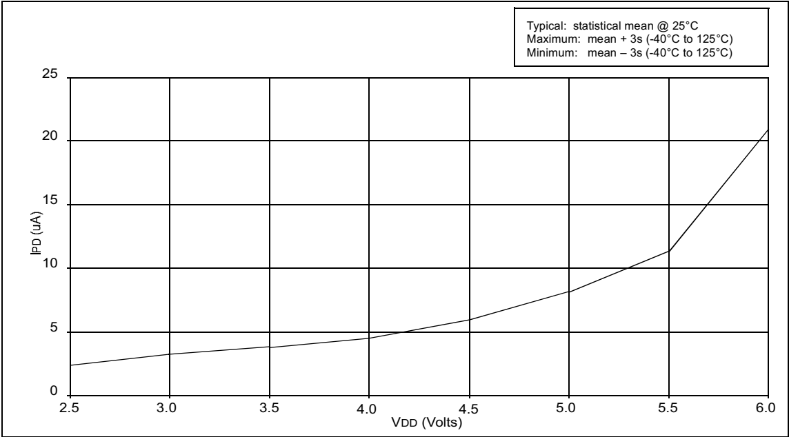
FIGURE 18-5: TYPICAL IPD vs. VDD, WATCHDOG DISABLED (25°C)
