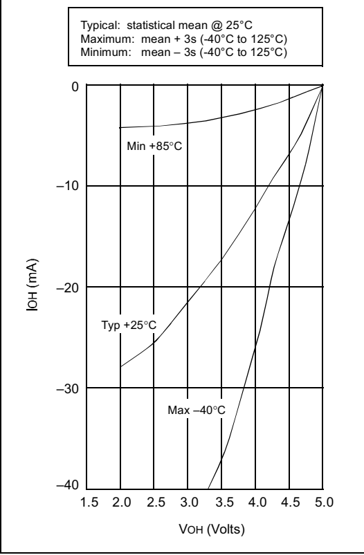
FIGURE 14-20: PORTA, B AND C I_{OH} vs. V_{OH} , V_{DD} = 5\text{ V}
