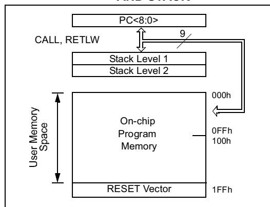
FIGURE 6-1: PIC16C54/CR54/C55 PROGRAM MEMORY MAP AND STACK
