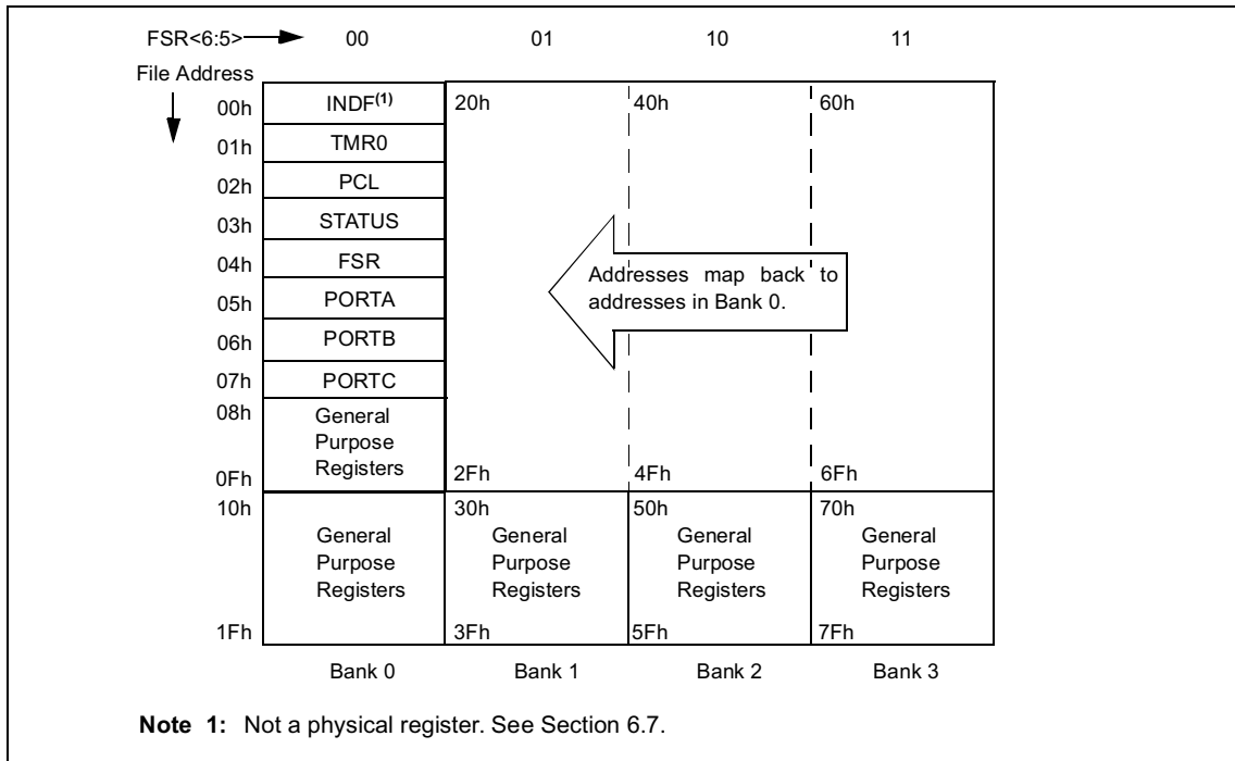
FIGURE 6-5: PIC16C57/CR57 REGISTER FILE MAP
