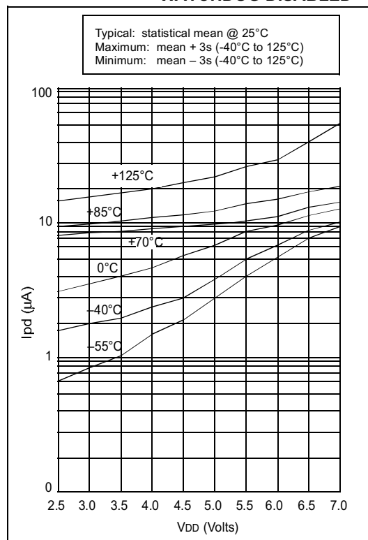
FIGURE 14-6: MAXIMUM IPD vs. VDD, WATCHDOG DISABLED
