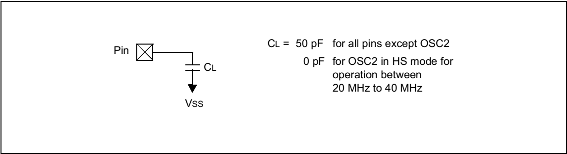
FIGURE 19-2: LOAD CONDITIONS FOR DEVICE TIMING SPECIFICATIONS - PIC16C54C/C55A/C56A/C57C/C58B-40
