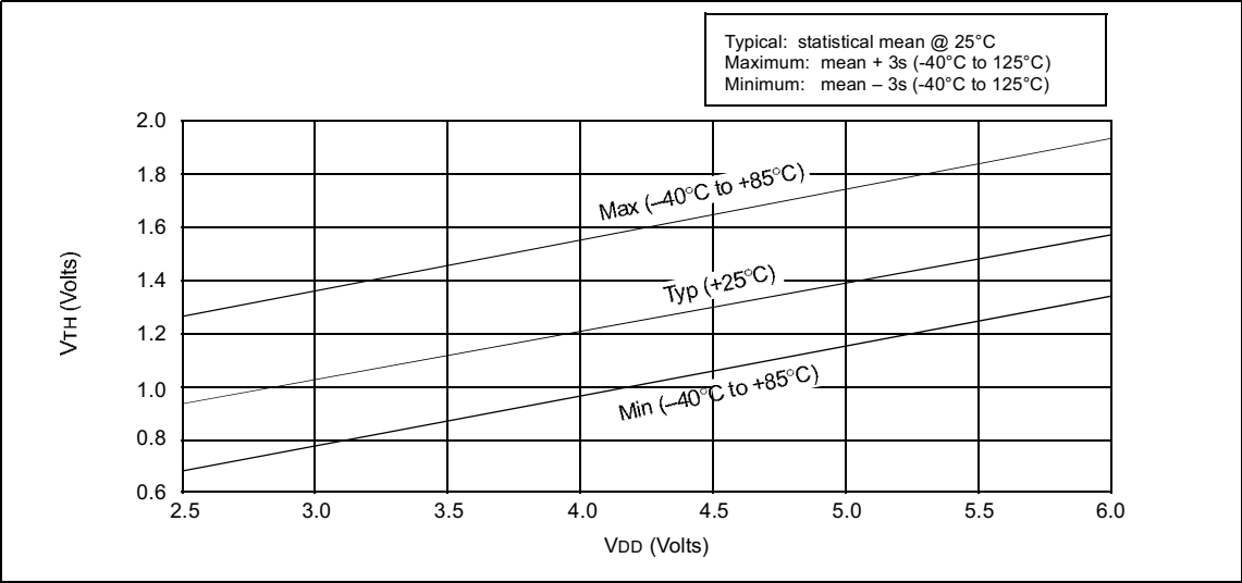
FIGURE 16-8: V_{TH} (INPUT THRESHOLD VOLTAGE) OF OSC1 INPUT (IN XT, HS, AND LP MODES) vs. V_{DD}
