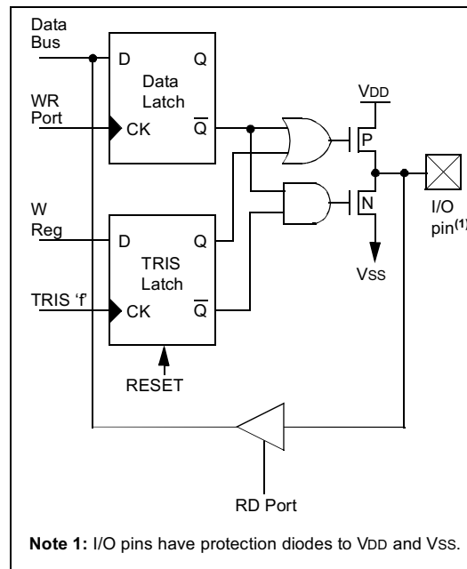
FIGURE 7-1: EQUIVALENT CIRCUIT FOR A SINGLE I/O PIN
