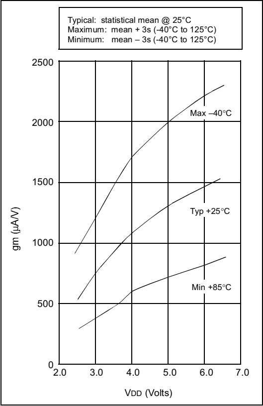
FIGURE 14-18: TRANSCONDUCTANCE (gm) OF XT OSCILLATOR vs. VDD
