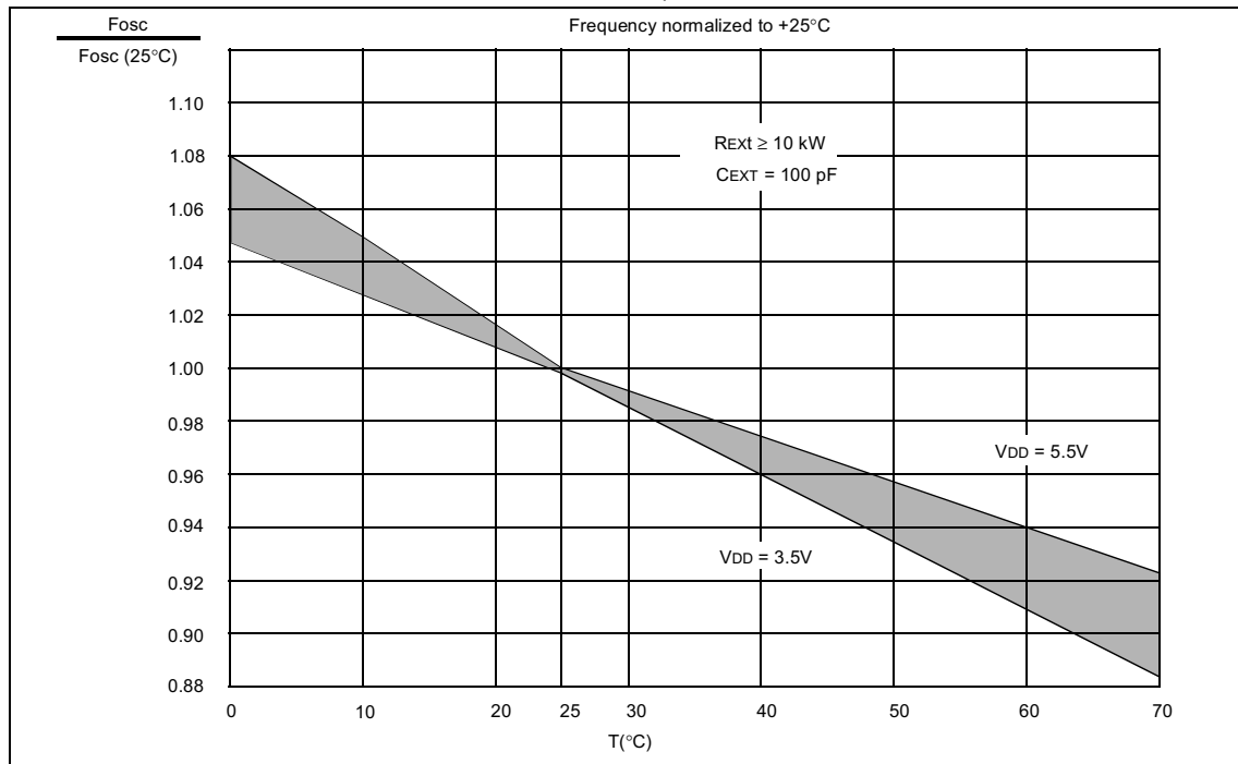
FIGURE 16-1: TYPICAL RC OSCILLATOR FREQUENCY vs. TEMPERATURE
