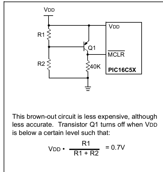
FIGURE 5-7: EXTERNAL BROWN-OUT PROTECTION CIRCUIT 2
