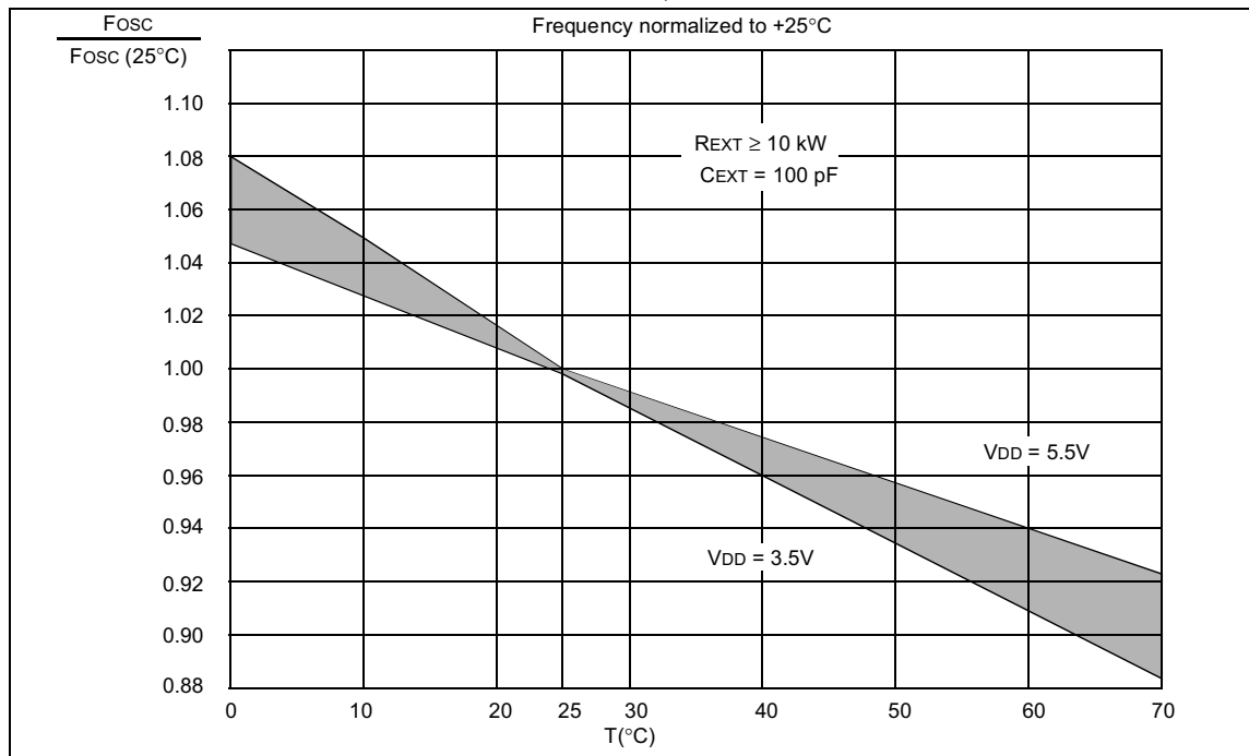
FIGURE 18-1: TYPICAL RC OSCILLATOR FREQUENCY vs. TEMPERATURE
