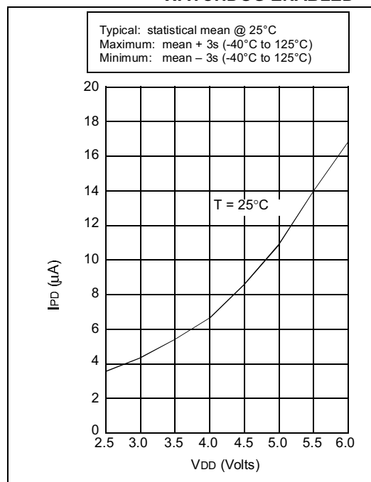
FIGURE 14-7: TYPICAL IPD vs. VDD, WATCHDOG ENABLED
