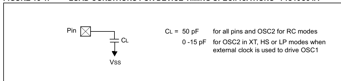
FIGURE 15-1: LOAD CONDITIONS FOR DEVICE TIMING SPECIFICATIONS - PIC16C54A
