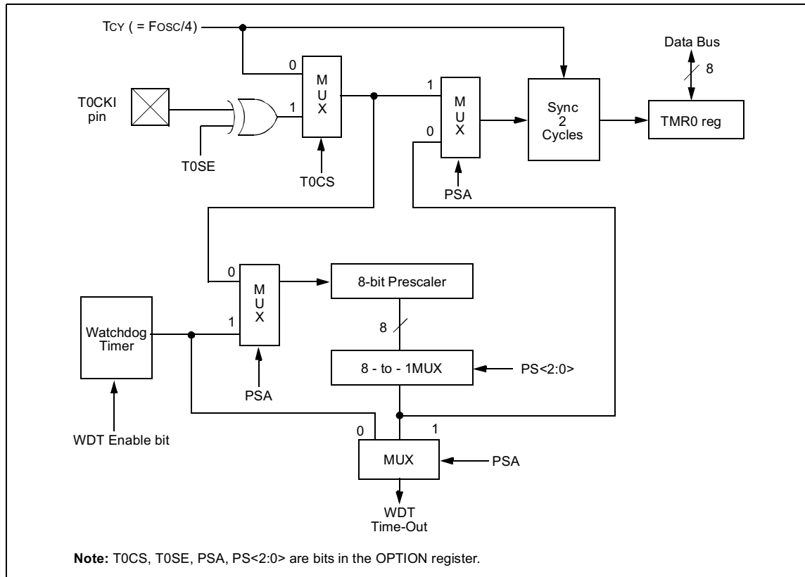
FIGURE 8-6: BLOCK DIAGRAM OF THE TIMER0/WDT PRESCALER
