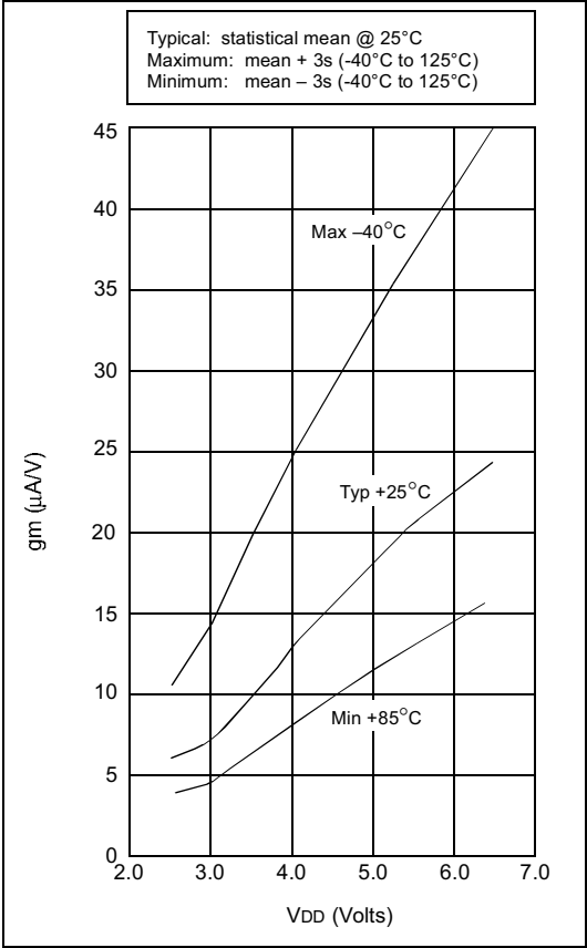
FIGURE 14-17: TRANSCONDUCTANCE (gm) OF LP OSCILLATOR vs. VDD
