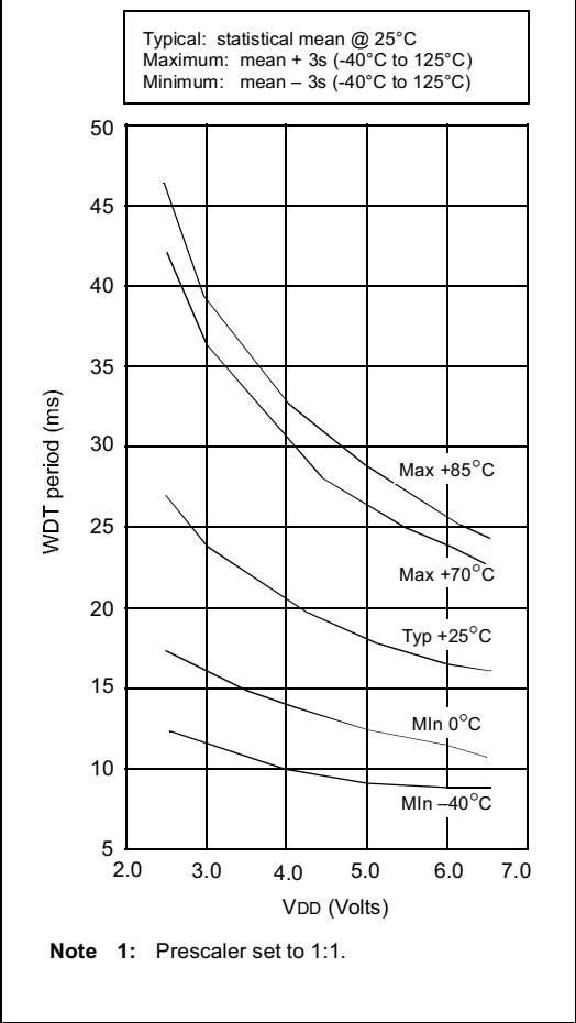
FIGURE 16-16: WDT TIMER TIME-OUT PERIOD vs. VDD (1)
