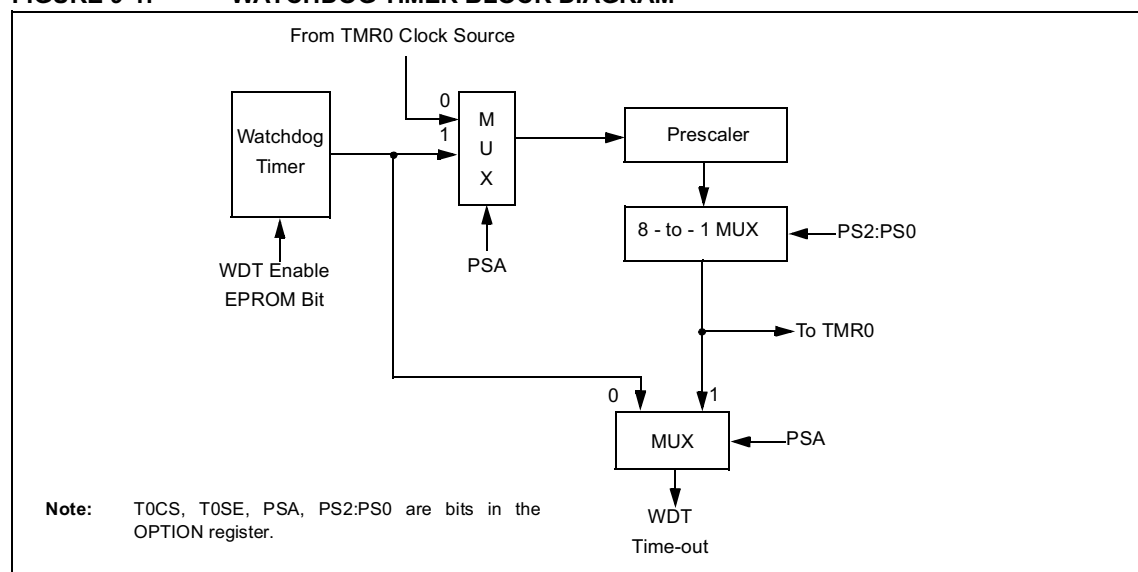
FIGURE 9-1: WATCHDOG TIMER BLOCK DIAGRAM
