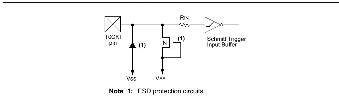
FIGURE 8-2: ELECTRICAL STRUCTURE OF T0CKI PIN
