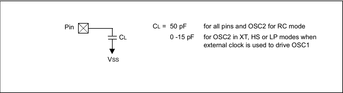
FIGURE 17-5: LOAD CONDITIONS FOR DEVICE TIMING SPECIFICATIONS - PIC16C54C/CR54C/C55A/C56A/CR56A/C57C/CR57C/C58B/CR58B-04, 20
