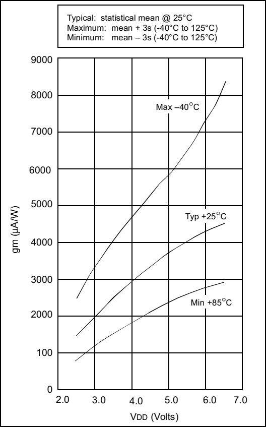
FIGURE 16-17: TRANSCONDUCTANCE (gm) OF HS OSCILLATOR vs. VDD
