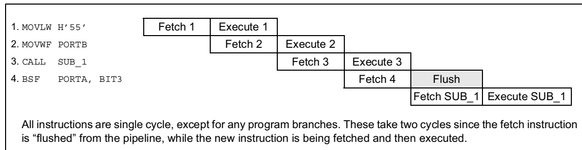
EXAMPLE 3-1: INSTRUCTION PIPELINE FLOW
