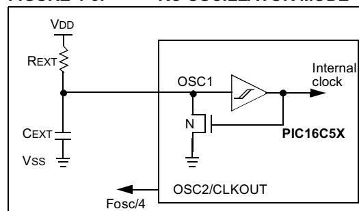
FIGURE 4-5: RC OSCILLATOR MODE
