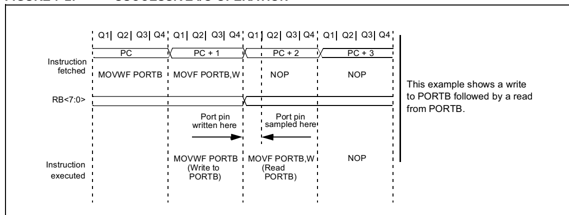
FIGURE 7-2: SUCCESSIVE I/O OPERATION
