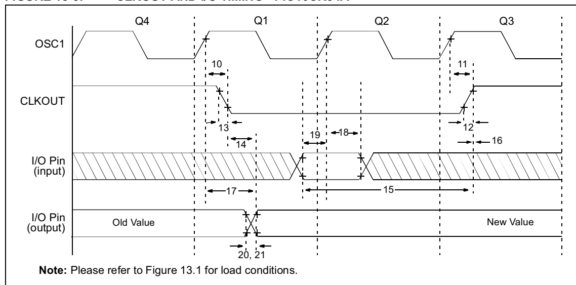
FIGURE 13-3: CLKOUT AND I/O TIMING - PIC16CR54A
