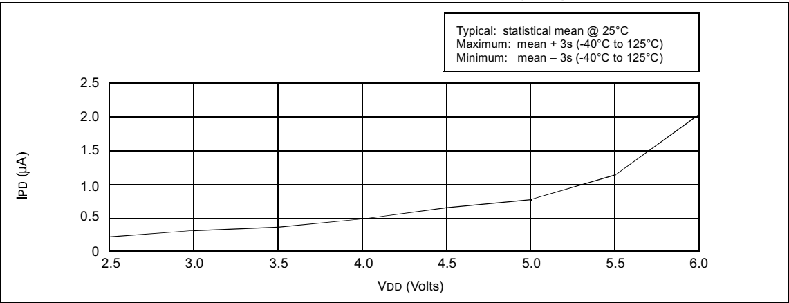
FIGURE 16-5: TYPICAL IPD vs. VDD, WATCHDOG DISABLED (25°C)
