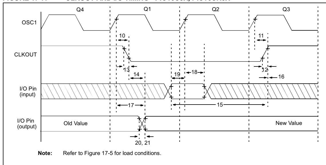
FIGURE 17-7: CLKOUT AND I/O TIMING - PIC16C5X, PIC16CR5X
