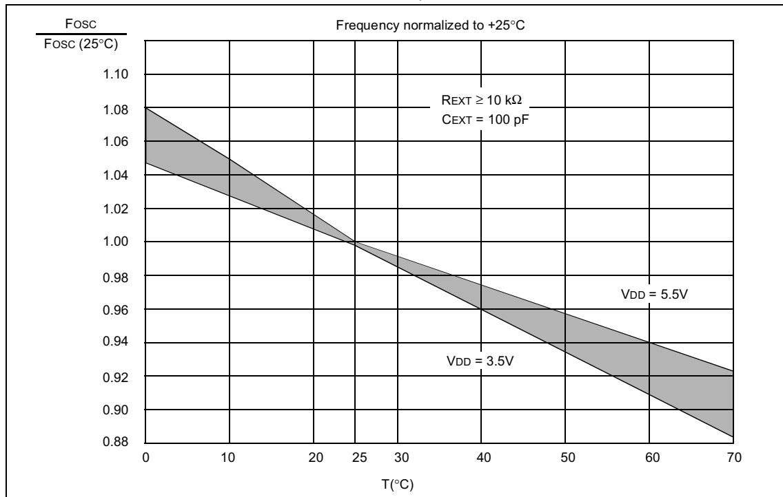
FIGURE 14-1: TYPICAL RC OSCILLATOR FREQUENCY vs. TEMPERATURE
