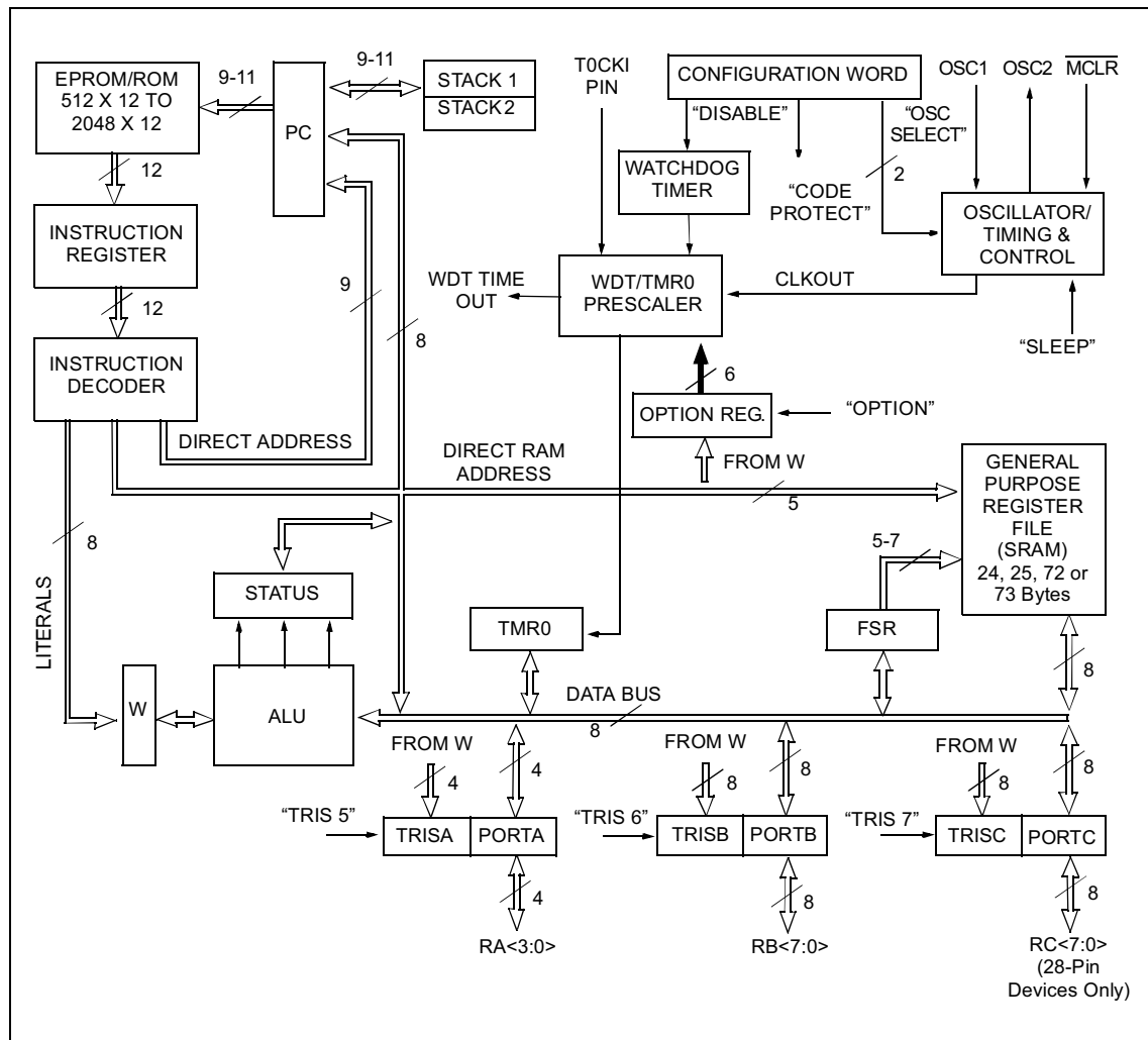
FIGURE 3-1: PIC16C5X SERIES BLOCK DIAGRAM
