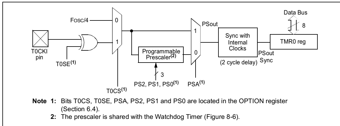
FIGURE 8-1: TIMER0 BLOCK DIAGRAM
