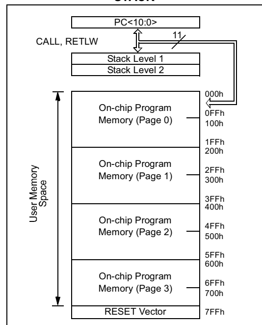
FIGURE 6-3: PIC16C57/CR57/C58/CR58 PROGRAM MEMORY MAP AND STACK
