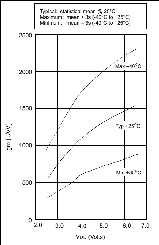
FIGURE 16-19: TRANSCONDUCTANCE (gm) OF XT OSCILLATOR vs. VDD
