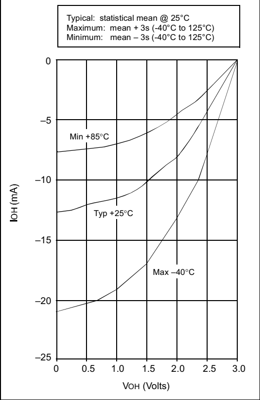
FIGURE 14-19: PORTA, B AND C I_{OH} vs. V_{OH} , V_{DD} = 3\text{ V}
