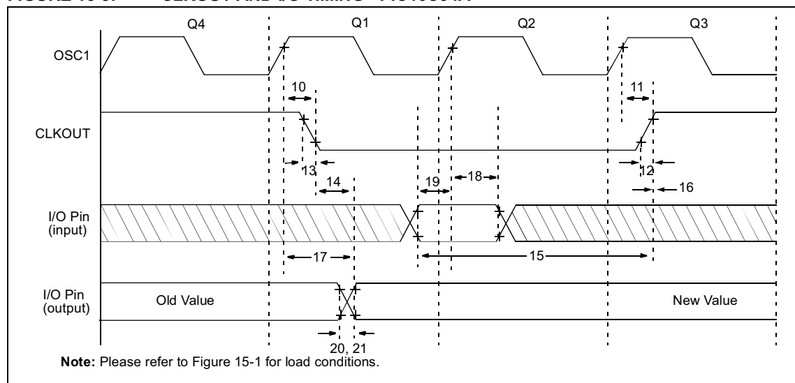
FIGURE 15-3: CLKOUT AND I/O TIMING - PIC16C54A
