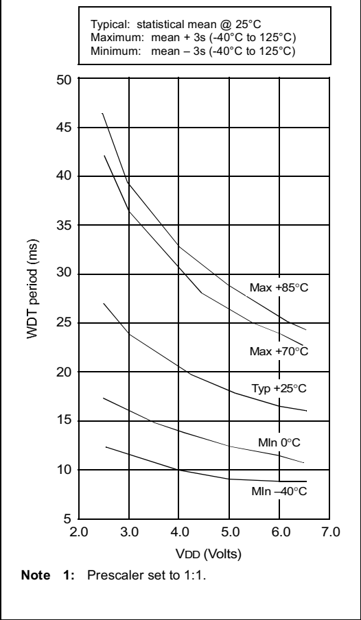
FIGURE 14-15: WDT TIMER TIME-OUT PERIOD vs. VDD (1)
