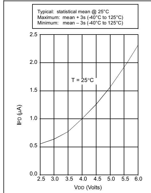
FIGURE 14-5: TYPICAL IPD vs. V DD , WATCHDOG DISABLED
