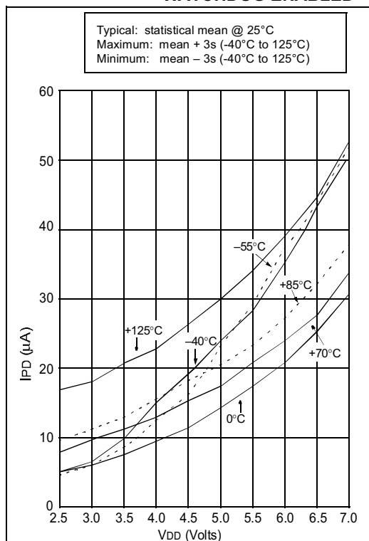
FIGURE 14-8: MAXIMUM IPD vs. VDD, WATCHDOG ENABLED
