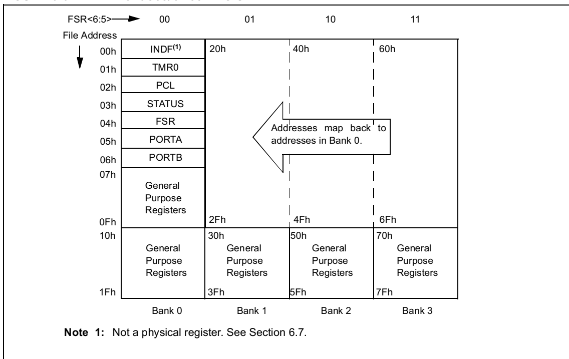
FIGURE 6-6: PIC16C58/CR58 REGISTER FILE MAP
