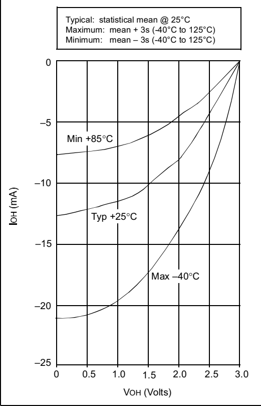
FIGURE 18-15: PORTA, B AND C I_{OH} vs. V_{OH} , V_{DD} = 3\text{ V}
