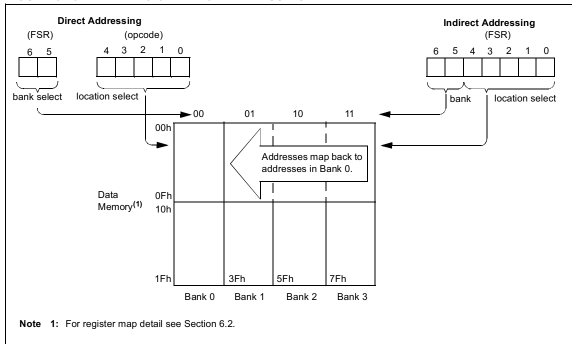
FIGURE 6-10: DIRECT/INDIRECT ADDRESSING
