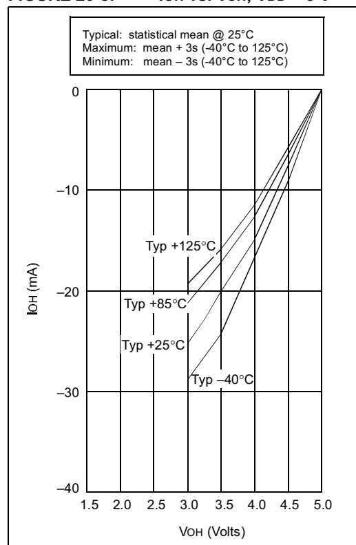
FIGURE 20-8: I_{OH} vs. V_{OH} , V_{DD} = 5\text{ V}
