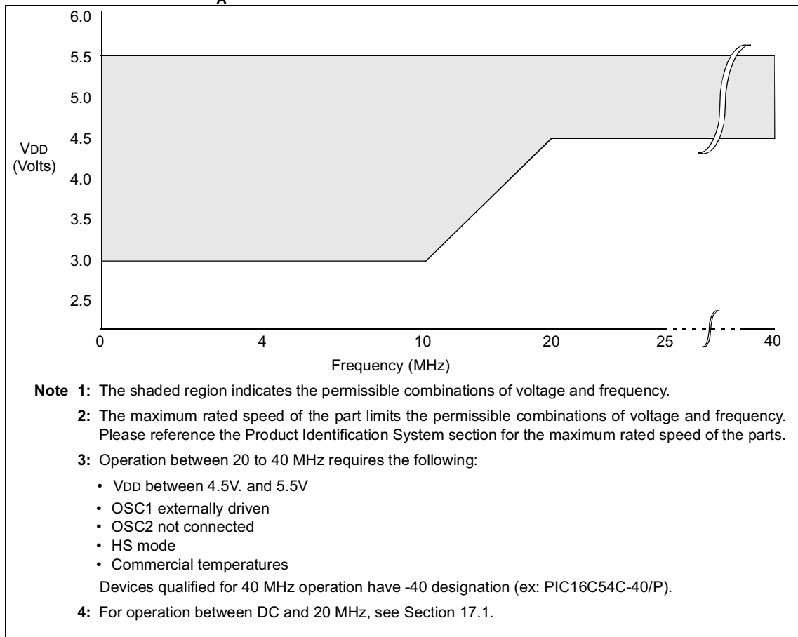
FIGURE 19-1: PIC16C54C/C55A/C56A/C57C/C58B-40 VOLTAGE-FREQUENCY GRAPH, 0^{\circ}\text{C} \leq T_A \leq +70^{\circ}\text{C}
