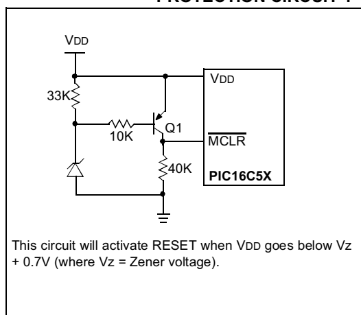
FIGURE 5-6: EXTERNAL BROWN-OUT PROTECTION CIRCUIT 1
