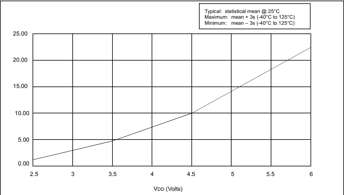
FIGURE 16-6: TYPICAL IPD vs. VDD, WATCHDOG ENABLED (25°C)
