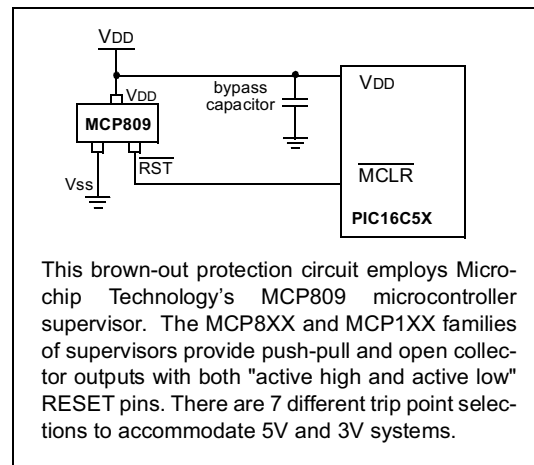
FIGURE 5-8: EXTERNAL BROWN-OUT PROTECTION CIRCUIT 3
