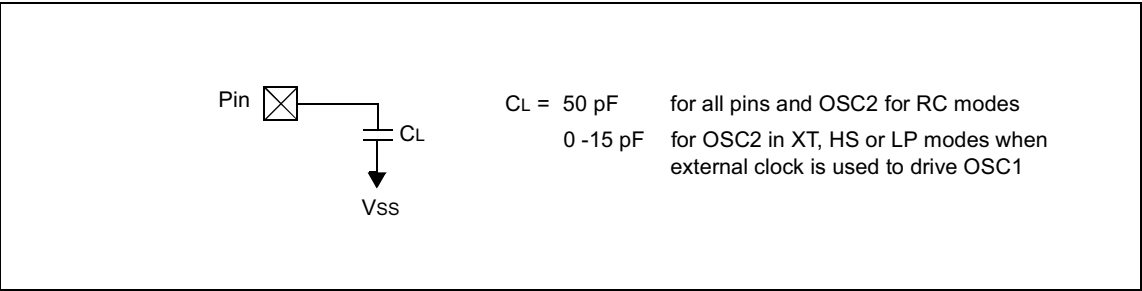
FIGURE 13-1: LOAD CONDITIONS FOR DEVICE TIMING SPECIFICATIONS - PIC16CR54A
