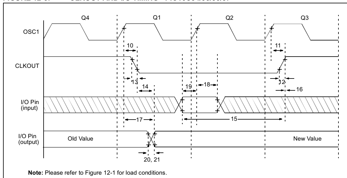
FIGURE 12-3: CLKOUT AND I/O TIMING - PIC16C54/55/56/57
