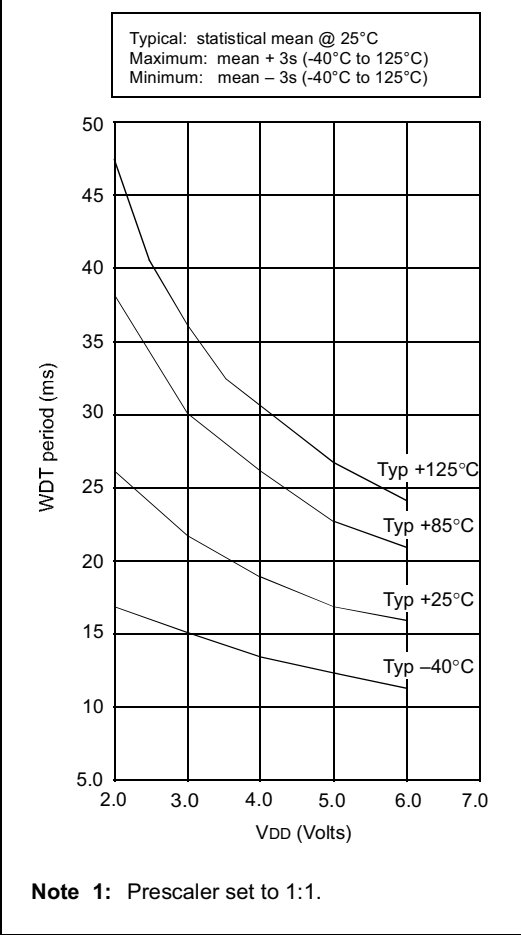
FIGURE 18-14: WDT TIMER TIME-OUT PERIOD vs. V_{DD}^{(1)}
