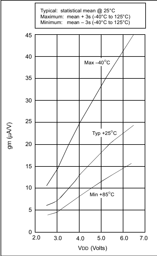
FIGURE 16-18: TRANSCONDUCTANCE (gm) OF LP OSCILLATOR vs. VDD
