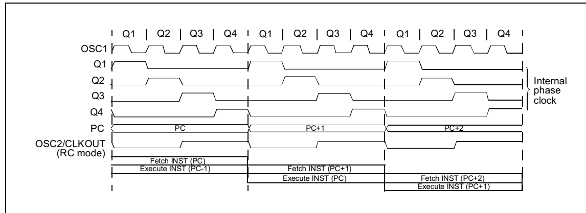
FIGURE 3-2: CLOCK/INSTRUCTION CYCLE
