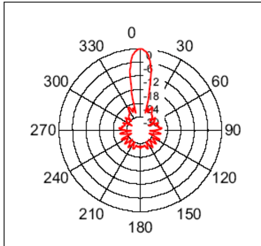
SRF235 Beam Pattern
