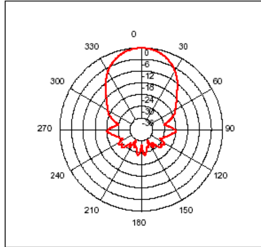
SRF04 Beam pattern
